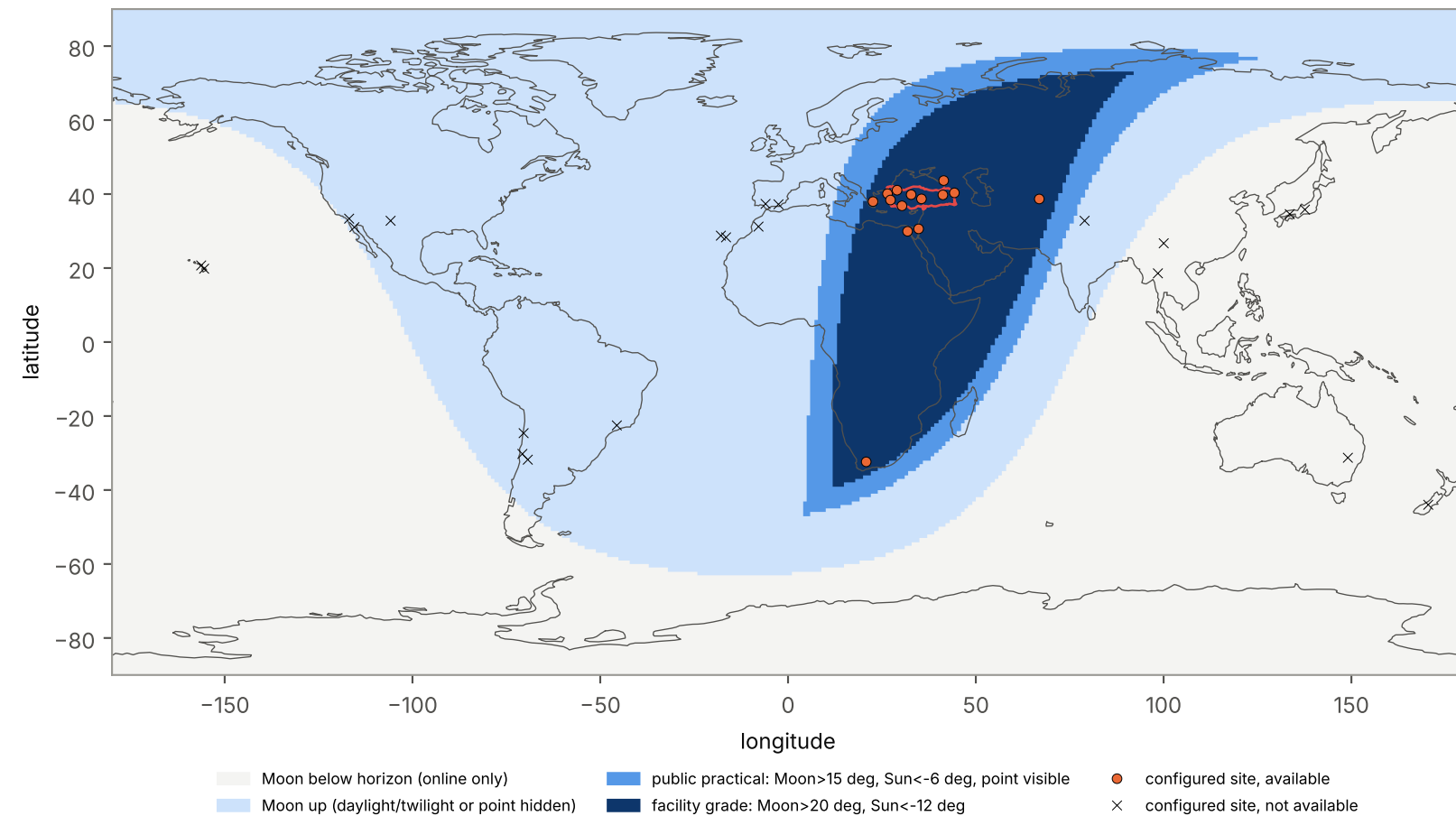
S8: Earth coverage at 2028-04-01 18:00 UTC, 2028-04-01 21:00 in Türkiye (UTC+3)
