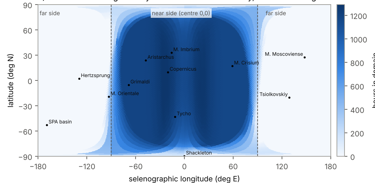
c) Hours with flash geometry and \geq 3 sites in dark sky, Moon > 20 deg
