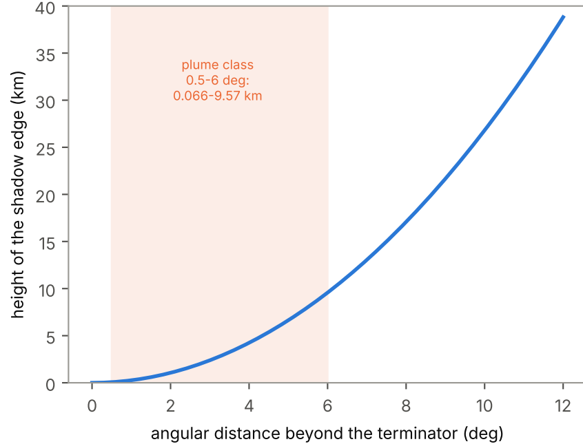
b) Height ejecta must reach to be sunlit (point Sun, sphere; the finite solar disc and terrain broaden the edge)
