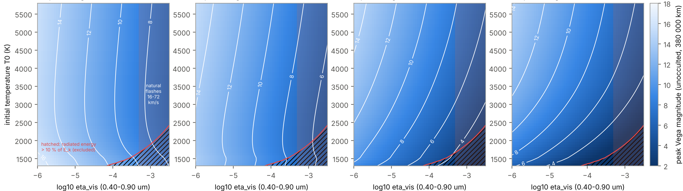
Rc peak magnitude
