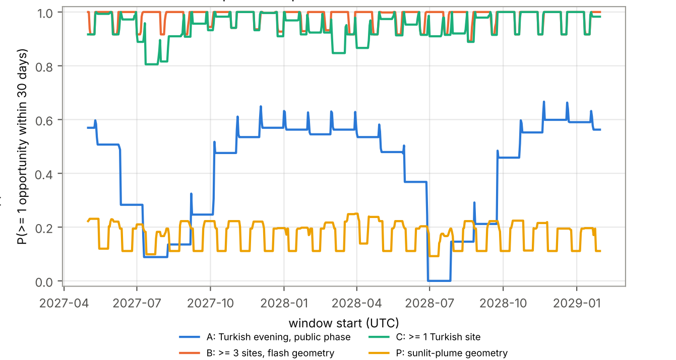
d) 30-day terminal window, cross-track \leq 0.6 deg, uniform over 72 directed planes x 8 phases
