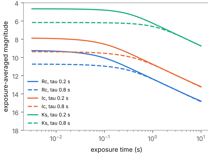
b) Dilution of the flash in longer exposures
