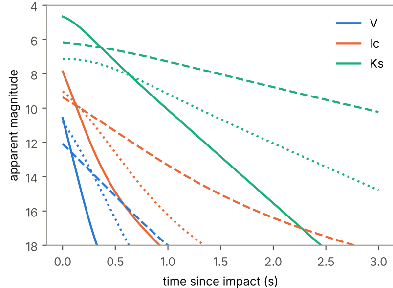
a) Model light curves, \eta_{\text{vis}} = 1e-4 (solid: 2500 K, \tau 0.2 s; dashed: 2500 K, 0.8 s; dotted: 3500 K, 0.4 s)
