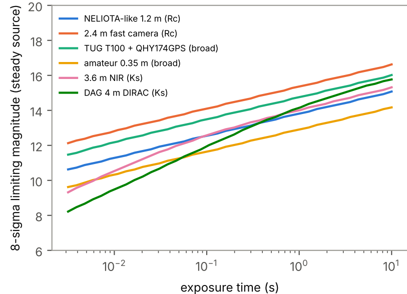
c) Above-atmosphere limits vs exposure (illum 0.35, 8' from sunlit terrain, dark sky, airmass 1.2 at 2500 m)
