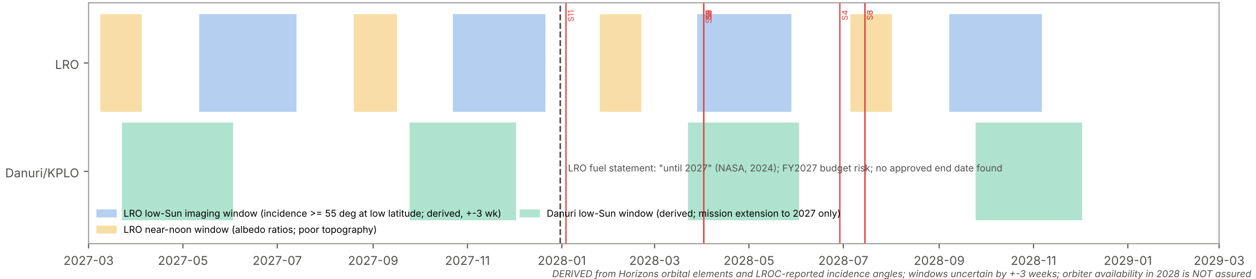
Orbiter follow-up: illumination windows (derived from the 331-day LRO beta cycle; research/orbiters.md) and scenario epochs
