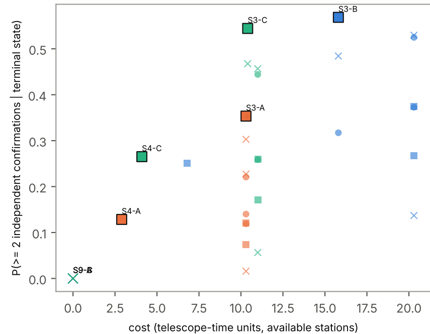
Strategy A/B/C objectives across hypothetical scenarios (wide luminous-efficiency prior; probabilities conditional on reaching the terminal state)
