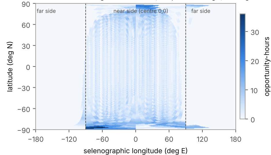
b) family average (24 node longitudes), no plane change
