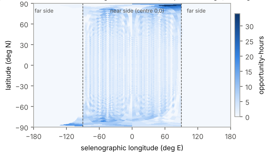
c) family average with a 2.5-deg cross-track budget (~70 m/s)
