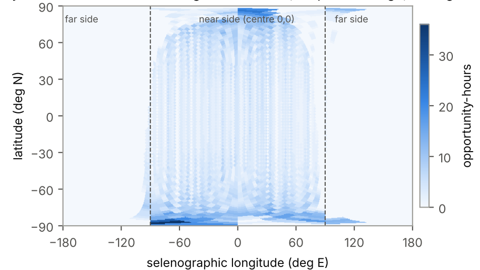
d) family average: flash geometry with \geq 3 configured sites anywhere
