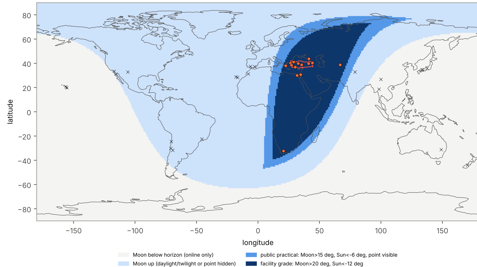
S2: Earth coverage at 2028-04-01 18:00:00 UTC (2028-04-01 21:00 (UTC+3)) - dots: configured sites (orange = available)
