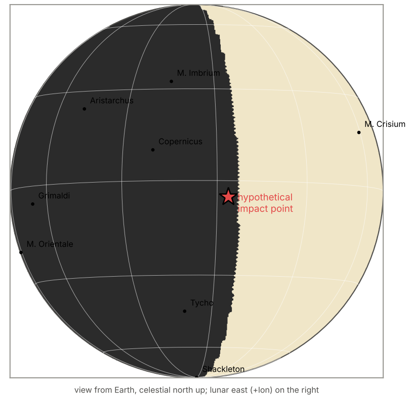
Moon at 2028-04-01 18:00 UTC: illuminated 39 %
