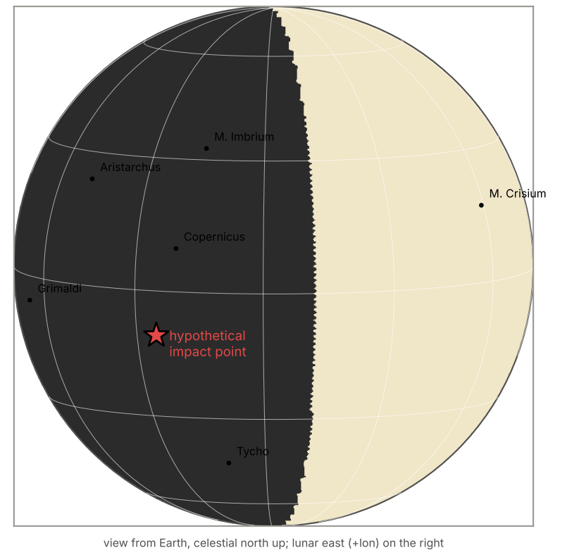
Moon at 2028-06-28 19:00 UTC: illuminated 42 %
