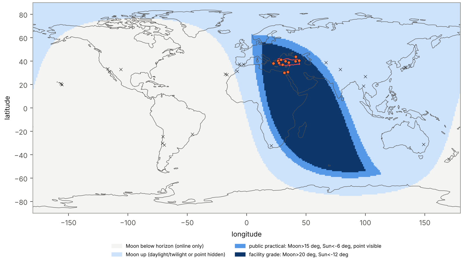
S6: Earth coverage at 2028-07-15 00:00:00 UTC (2028-07-15 03:00 (UTC+3)) - dots: configured sites (orange = available)
