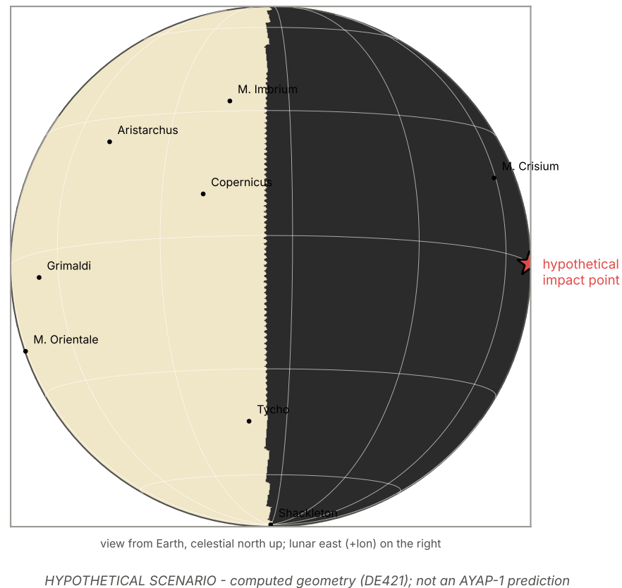
Moon at 2028-07-15 00:00 UTC: illuminated 49 %
