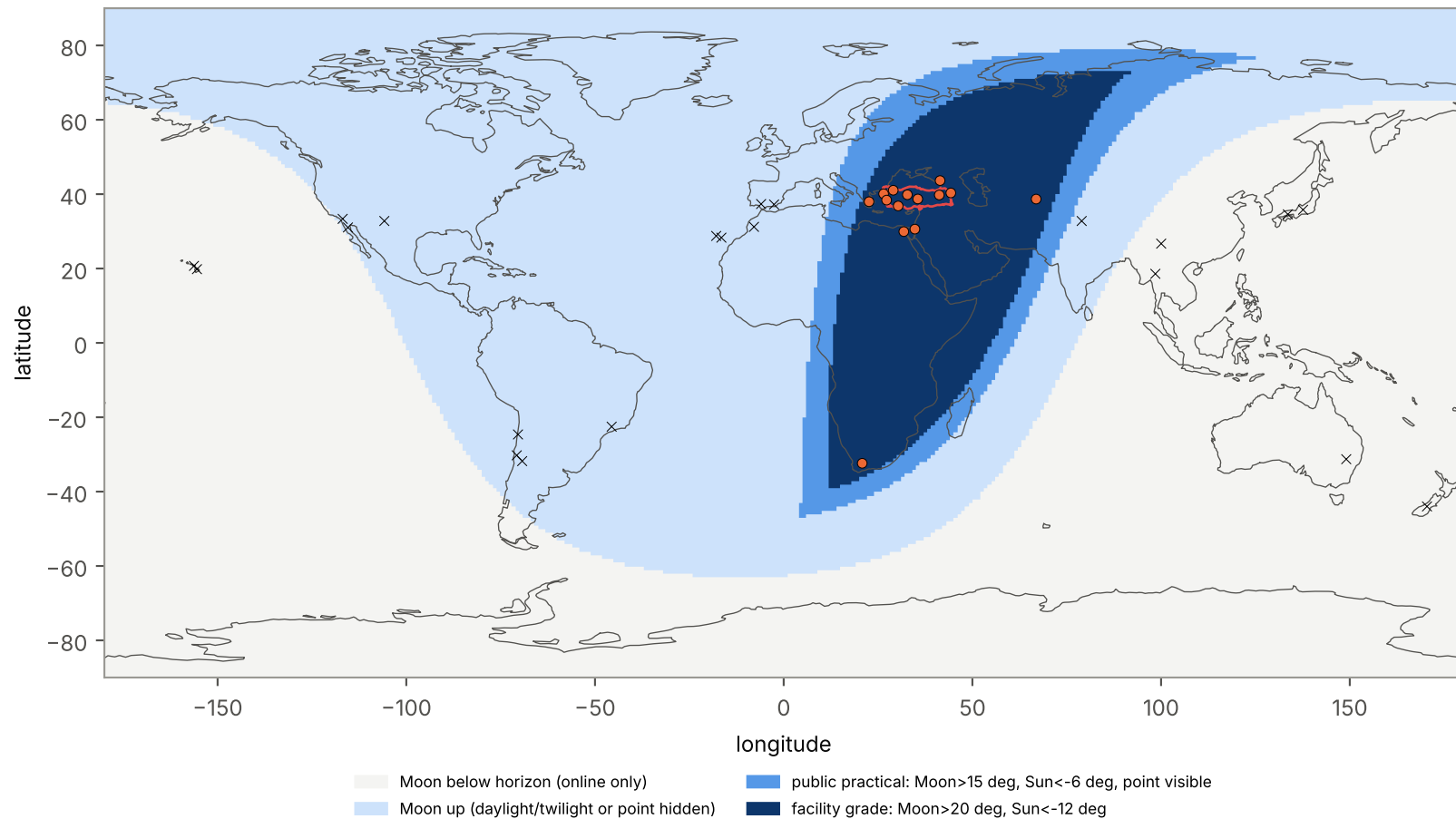
S8: Earth coverage at 2028-04-01 18:00:00 UTC (2028-04-01 21:00 (UTC+3)) - dots: configured sites (orange = available)
