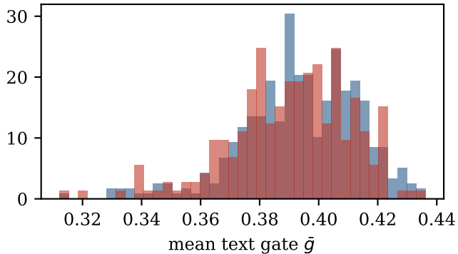
Rahutomo-600 (cross-dataset)
