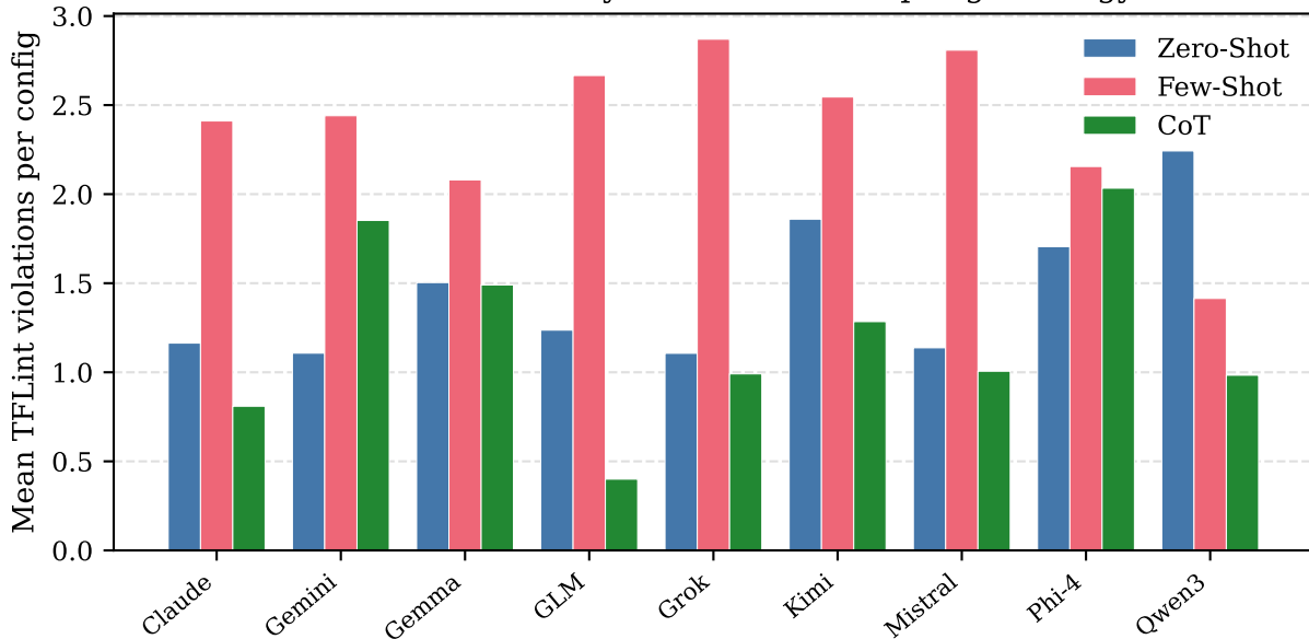
TFLint Violations by Model and Prompting Strategy
