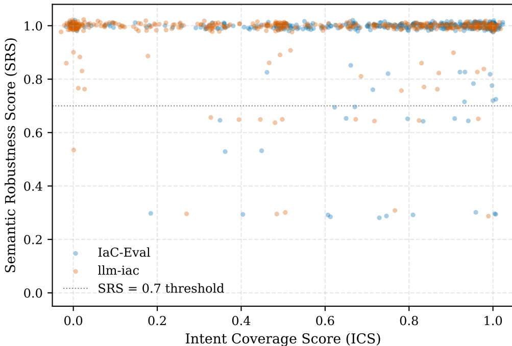
ICS vs. SRS per Prompt
