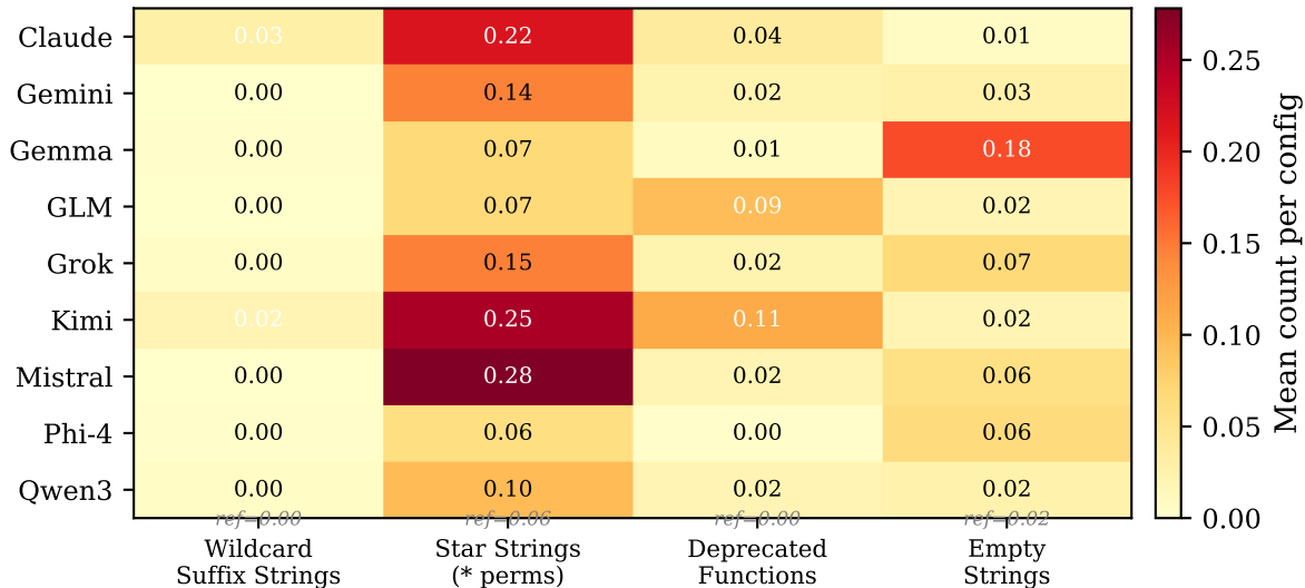
Risk Indicators per Model — IaC-Eval, Zero-Shot (TerraMetrics)
