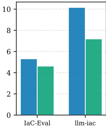
Num Resources
