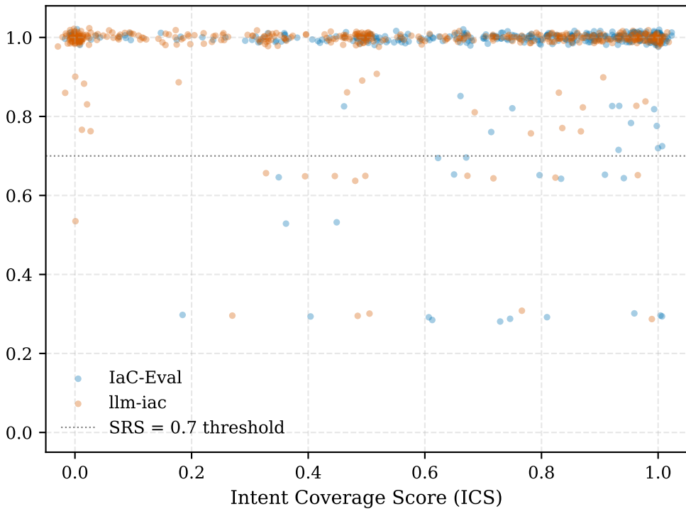
Semantic Robustness Score (SRS)
