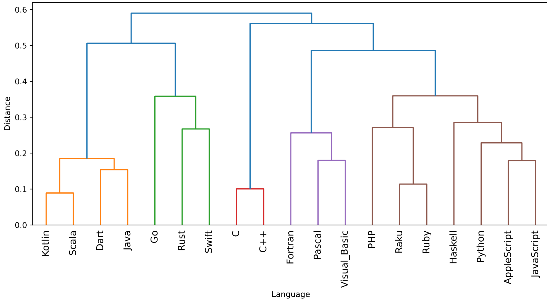
Hierarchical Clustering - octen CCC: 0.6162
