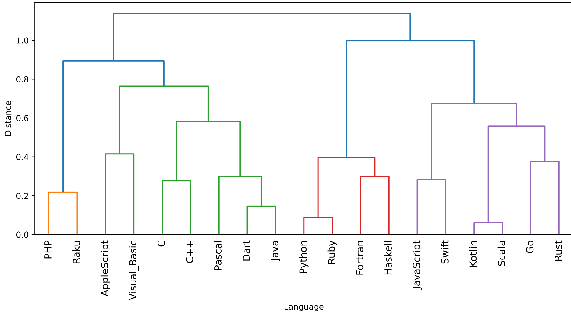
Hierarchical Clustering - minilm CCC: 0.6289
