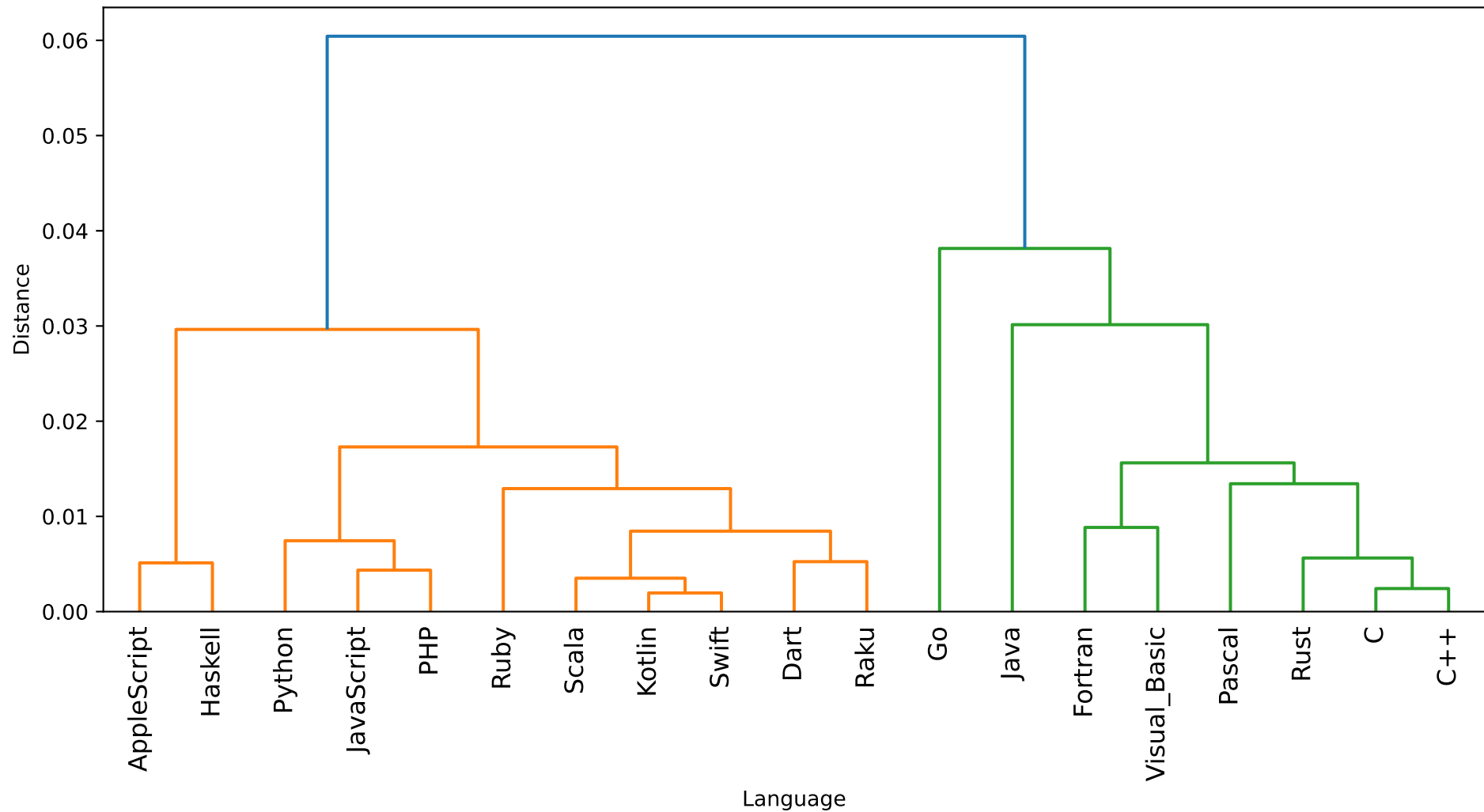
Hierarchical Clustering - codebert CCC: 0.5844
