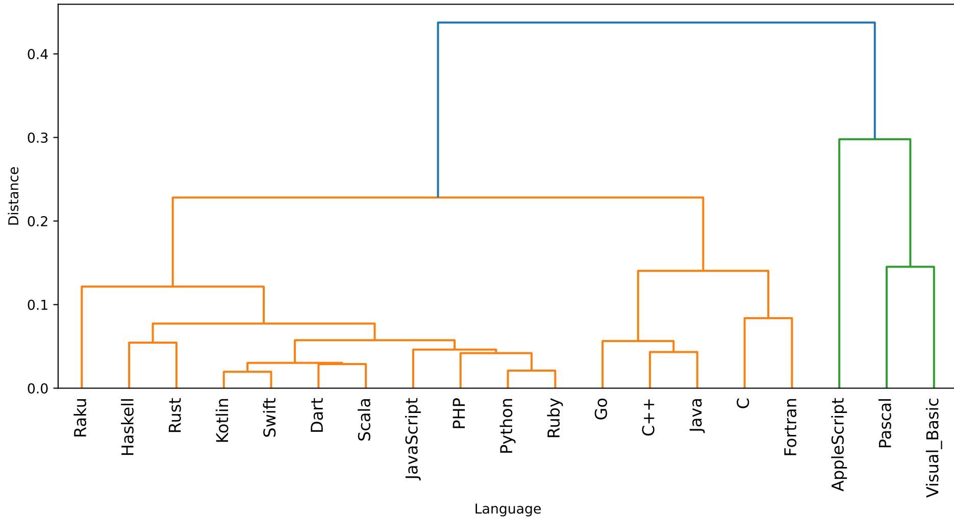
Hierarchical Clustering - jina_code CCC: 0.8509
