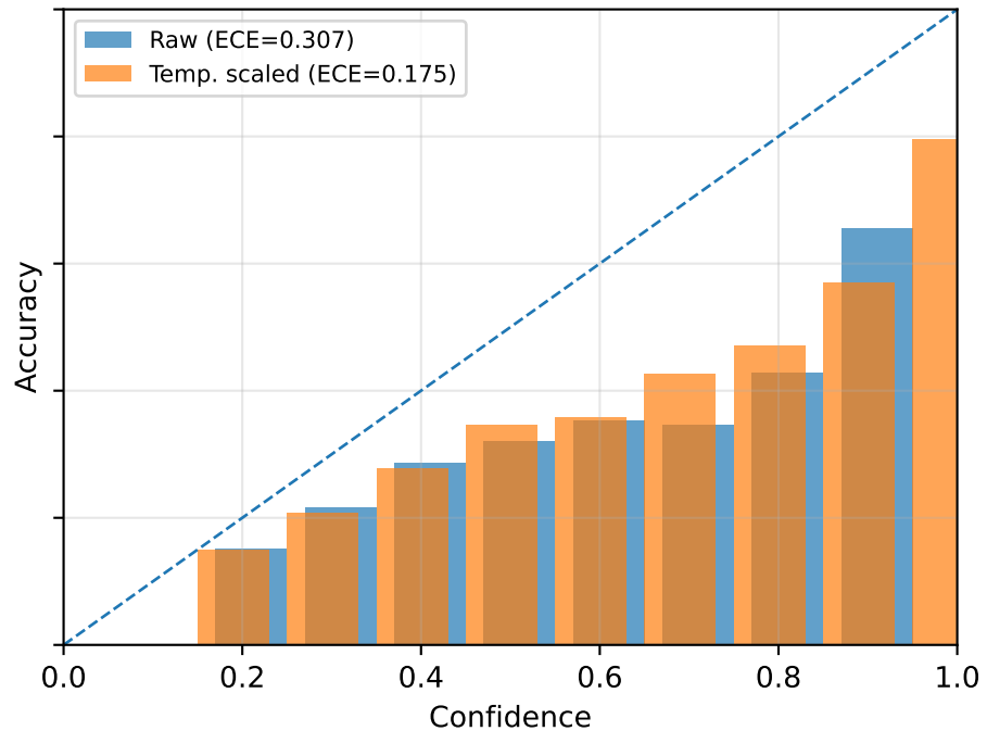
User 1, BiGRU + Proto(0.001)
