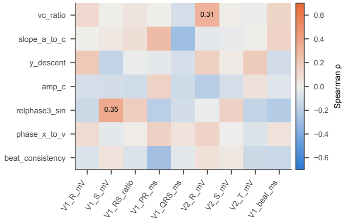
b JVP-ECG feature coupling (values: p < 0.05 )
