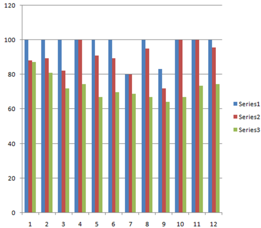
Figure 4.11: Series1 shows line segmentation, series2 shows word segmentation and series3 shows character segmentation.
