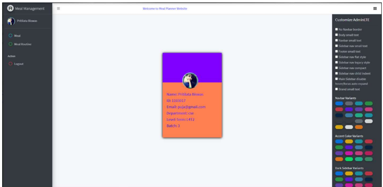
Figure 3.5: Student profile.
