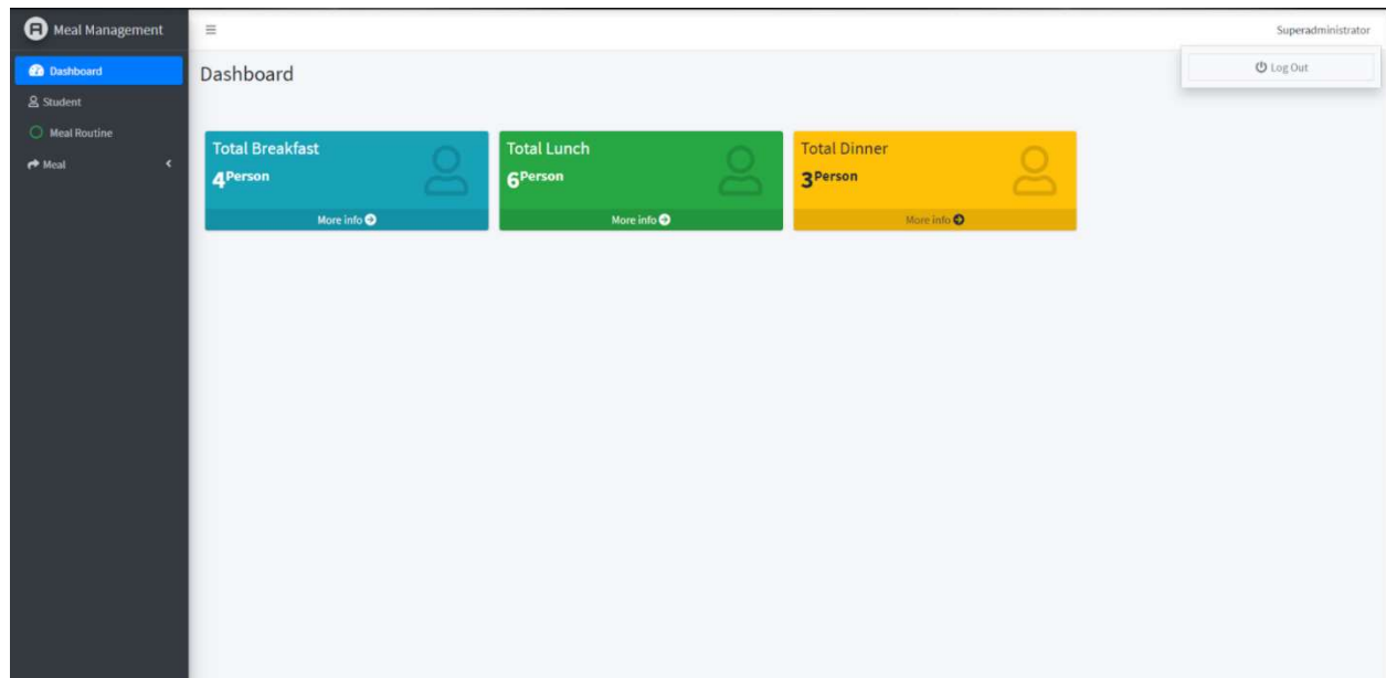
Figure 3.3: Admin dashboard.
