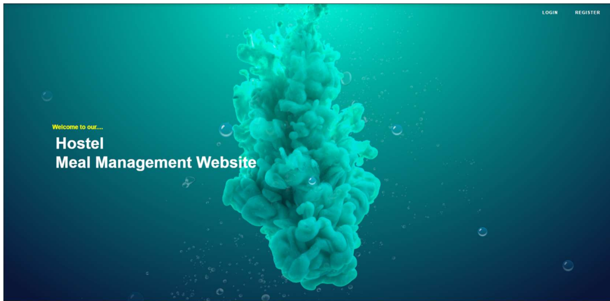
Figure 3.2: Homepage.
