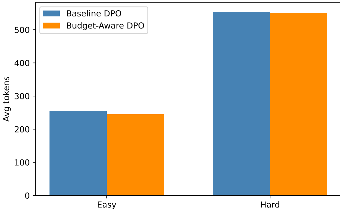
Avg Response Length by Complexity
