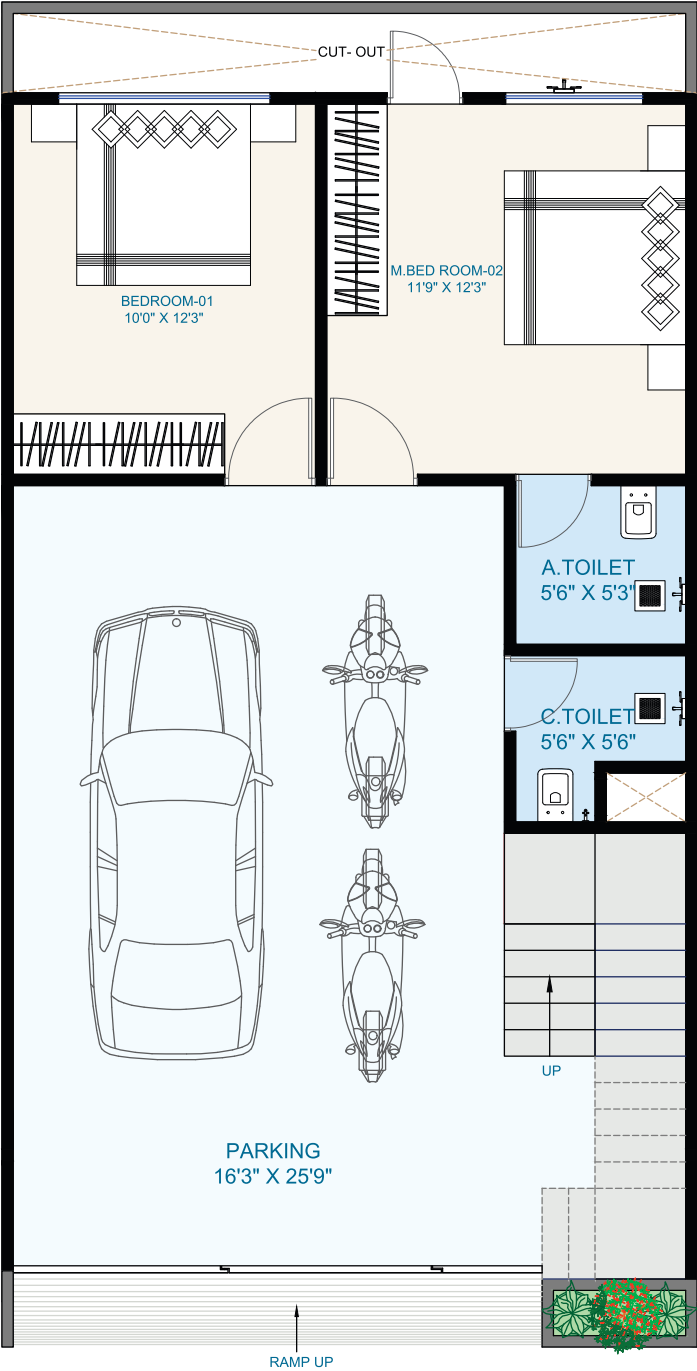
GROUND FLOOR PLAN FLOOR HEIGHT-10'-0"
