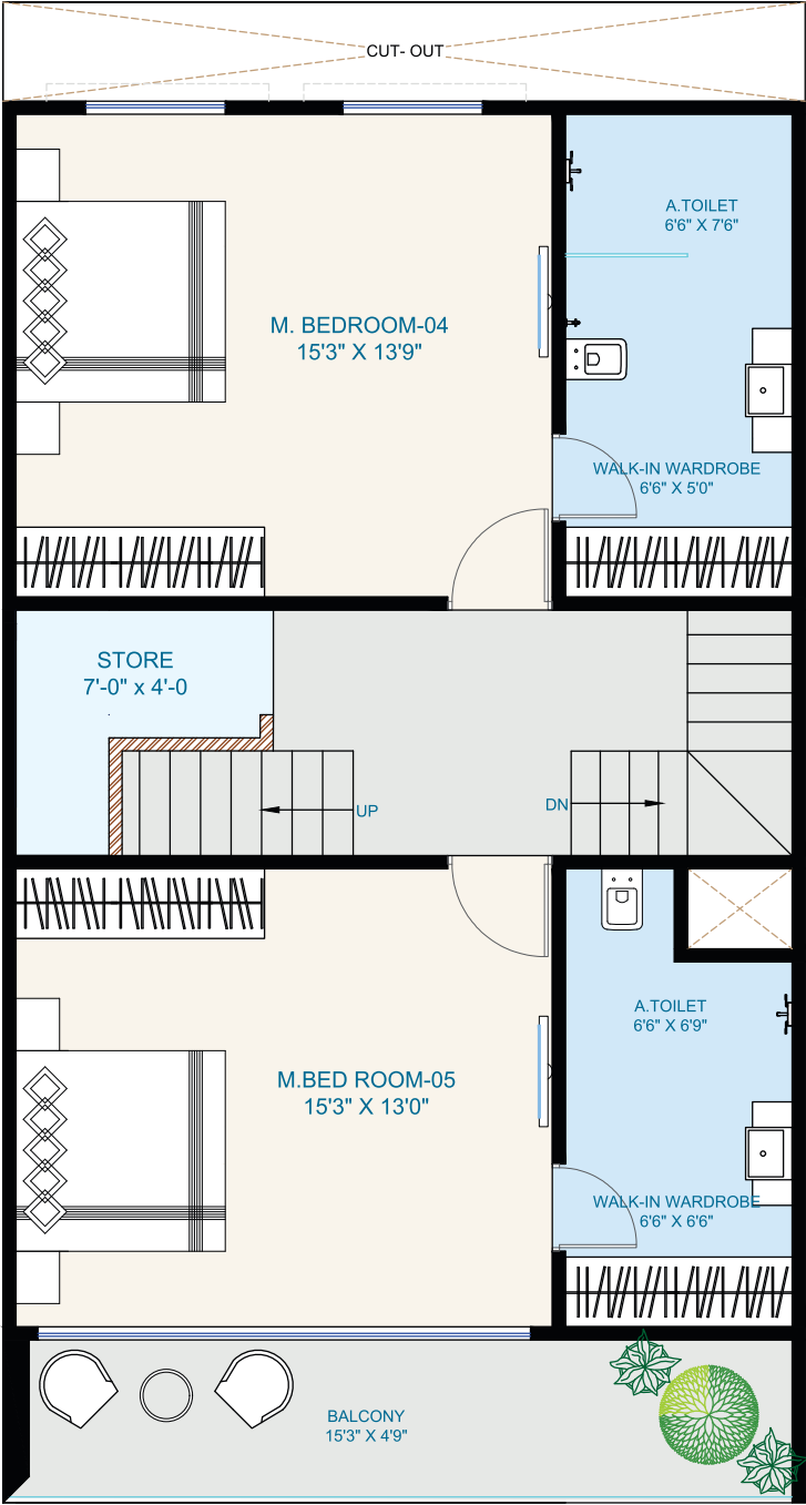
SECOND FLOOR PLAN FLOOR HEIGHT-10'-0"
