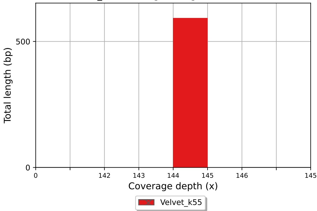
Velvet_k55 coverage histogram (bin size: 1x)
