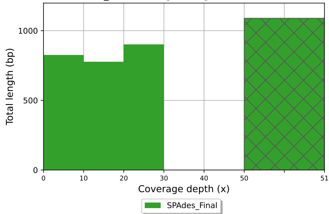
SPAdes_Final coverage histogram (bin size: 10x)
