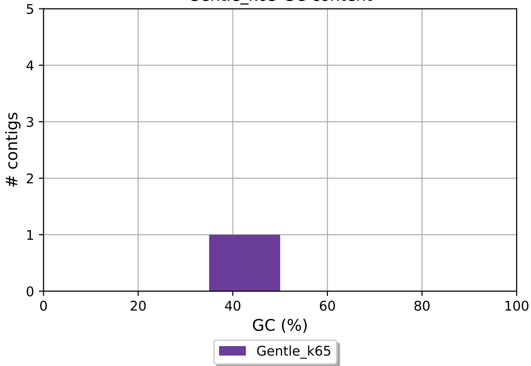
Gentle_k65 GC content
