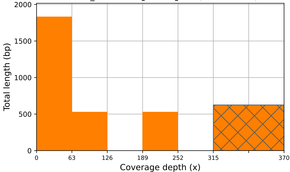
Gentle_k75 coverage histogram (bin size: 63x)
