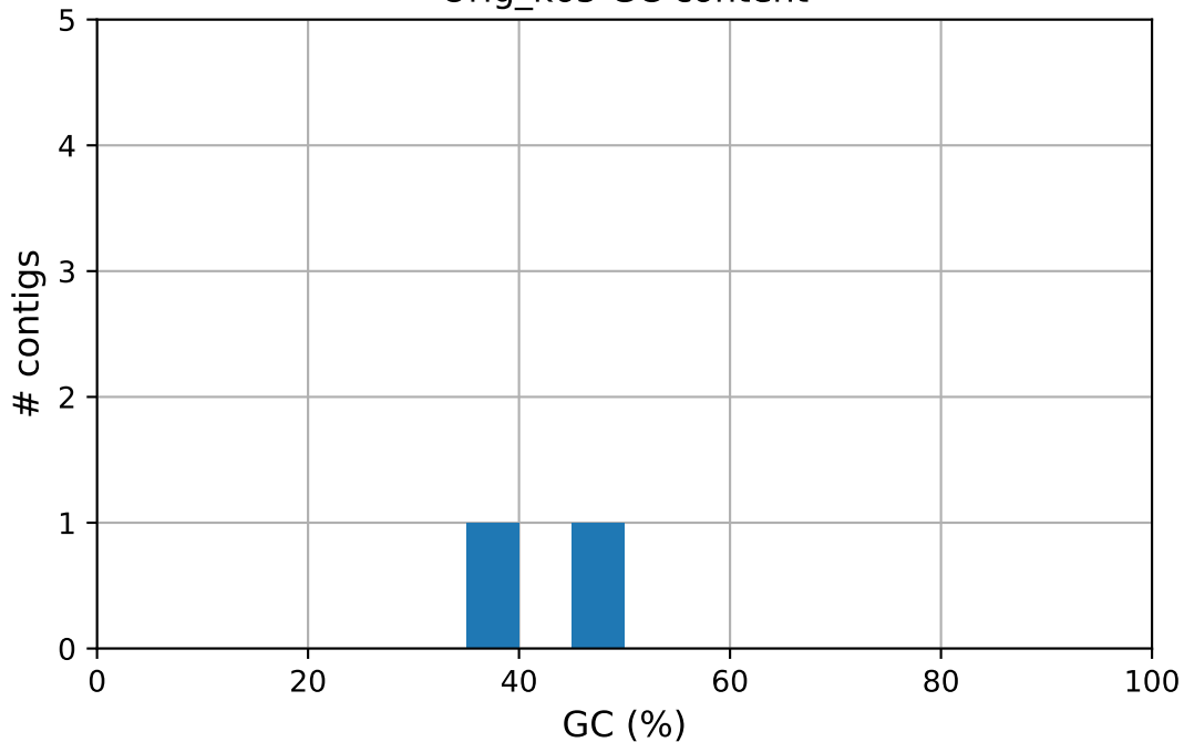
Orig_k65 GC content
