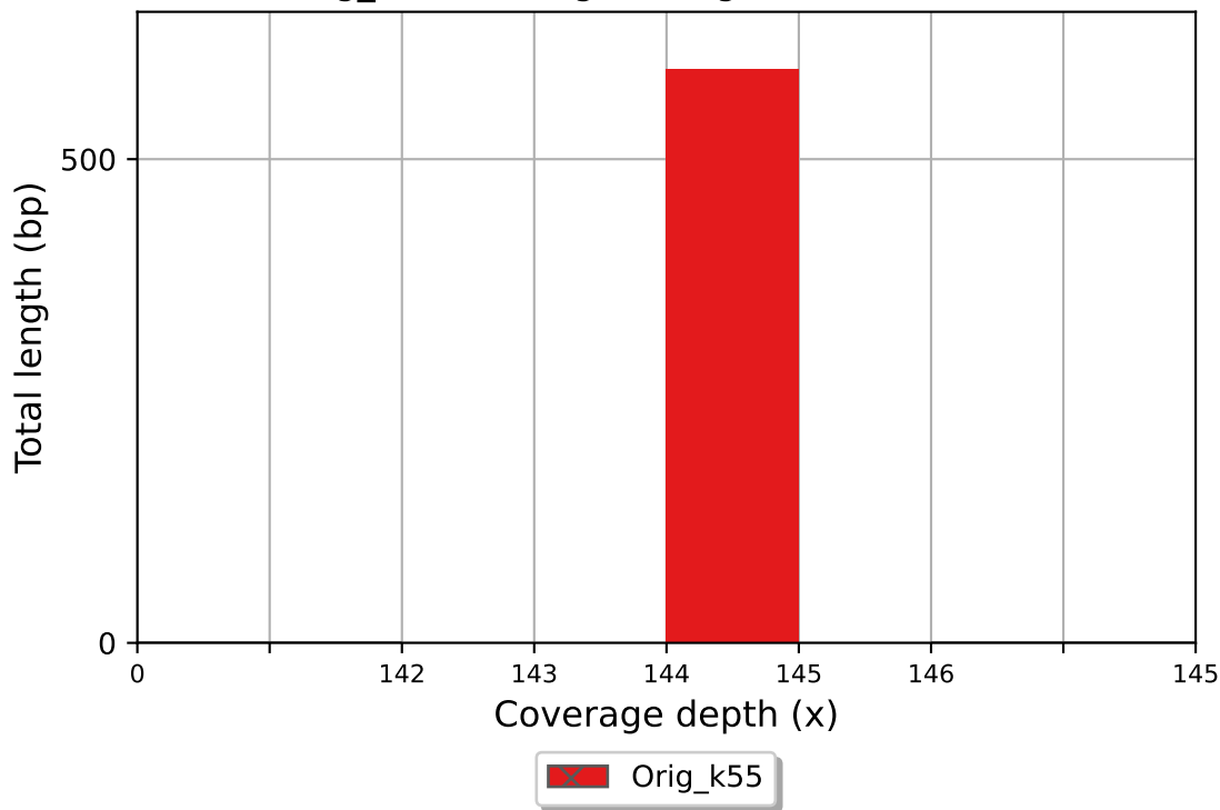
Orig_k55 coverage histogram (bin size: 1x)
