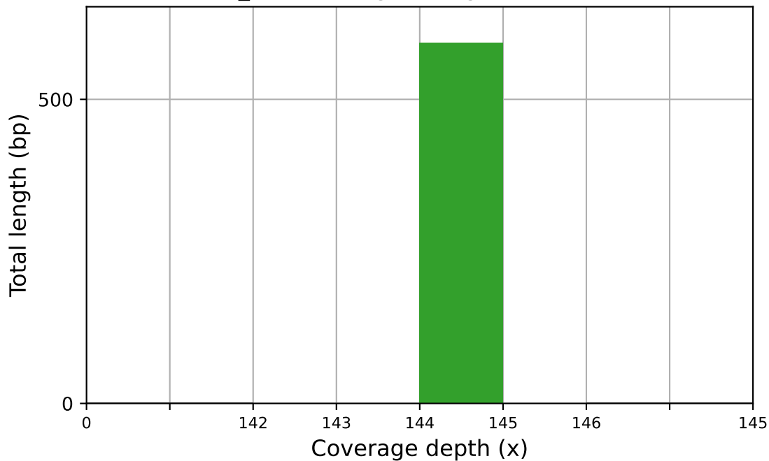
Gentle_k55 coverage histogram (bin size: 1x)
