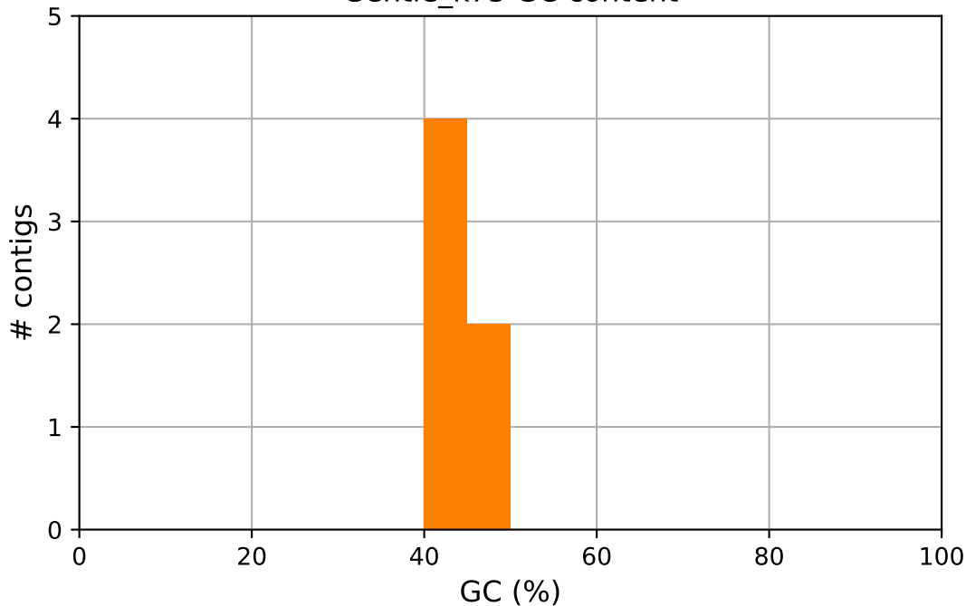
Gentle_k75 GC content
