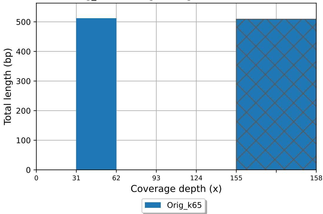
Orig_k65 coverage histogram (bin size: 31x)
