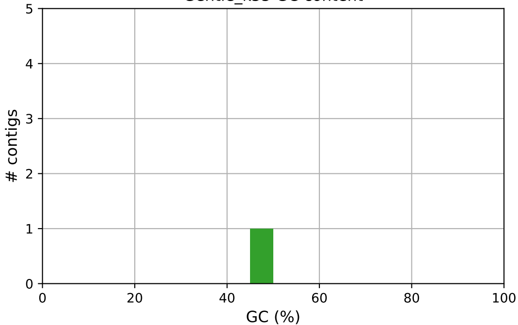
Gentle_k55 GC content
