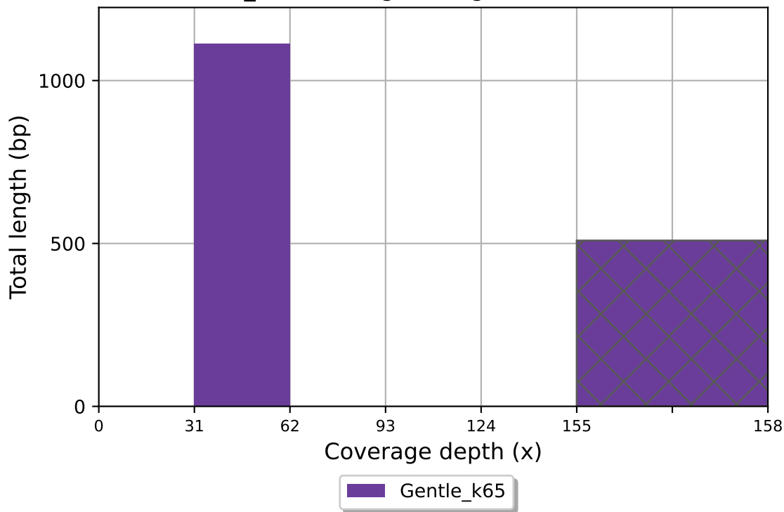
Gentle_k65 coverage histogram (bin size: 31x)
