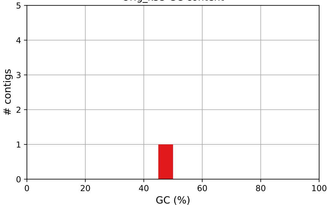
Orig_k55 GC content
