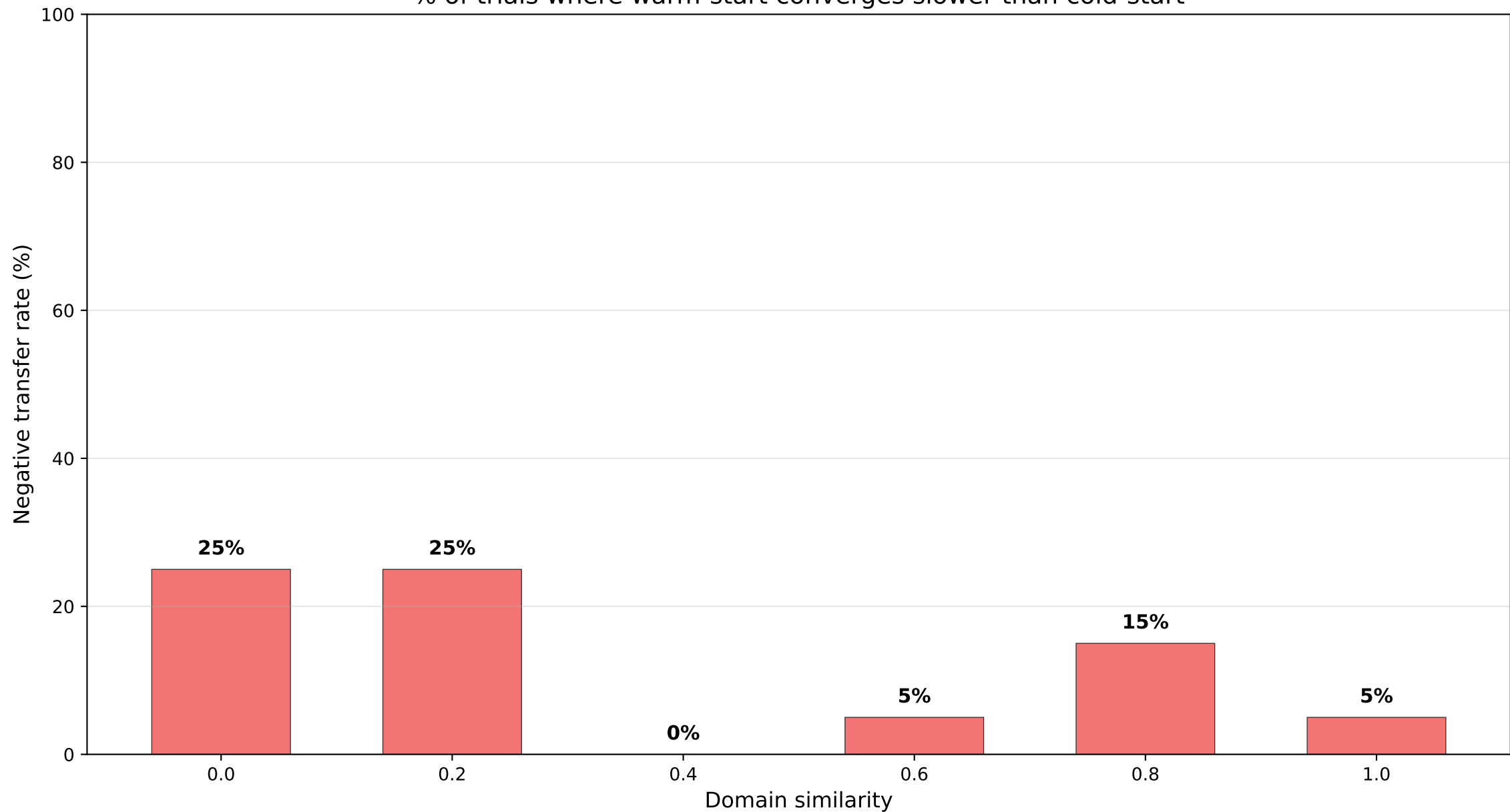
E-JM-3: When Does Transfer HURT? % of trials where warm-start converges slower than cold-start
