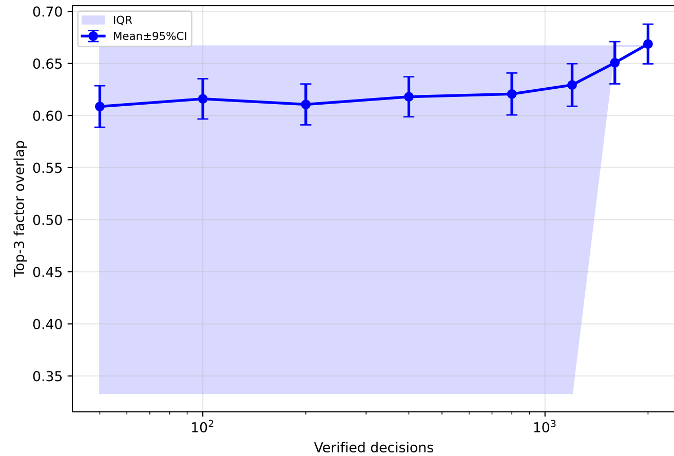
E-JM-5 v2: DK Weight Convergence (100 domains × 5 trials)
