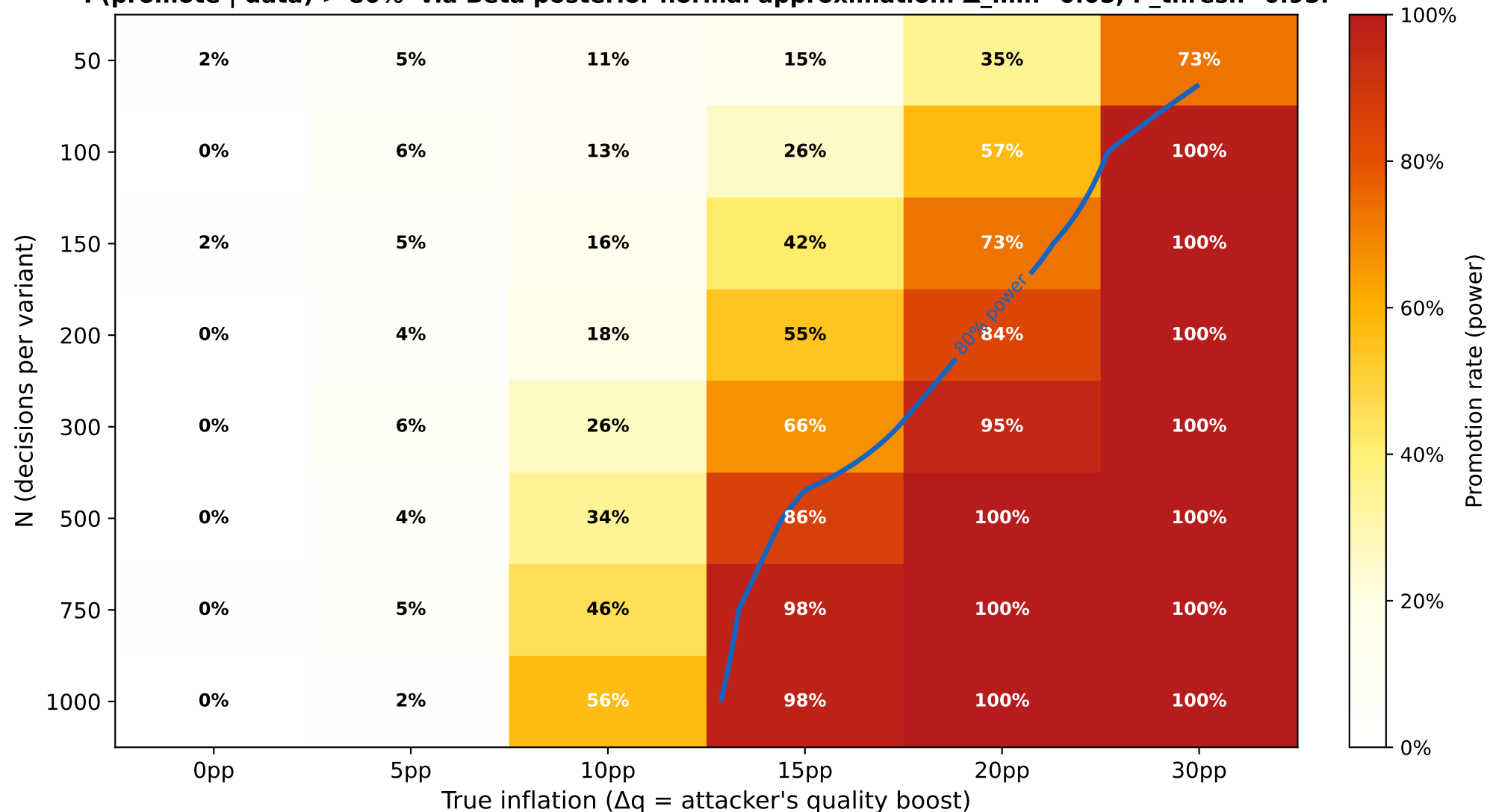
Gate 1 Detection Power: N vs Inflation P(\text{promote} \mid \text{data}) > 80\% via Beta posterior normal approximation. \Delta_{\min}=0.05 , P_{\text{thresh}}=0.95 .
