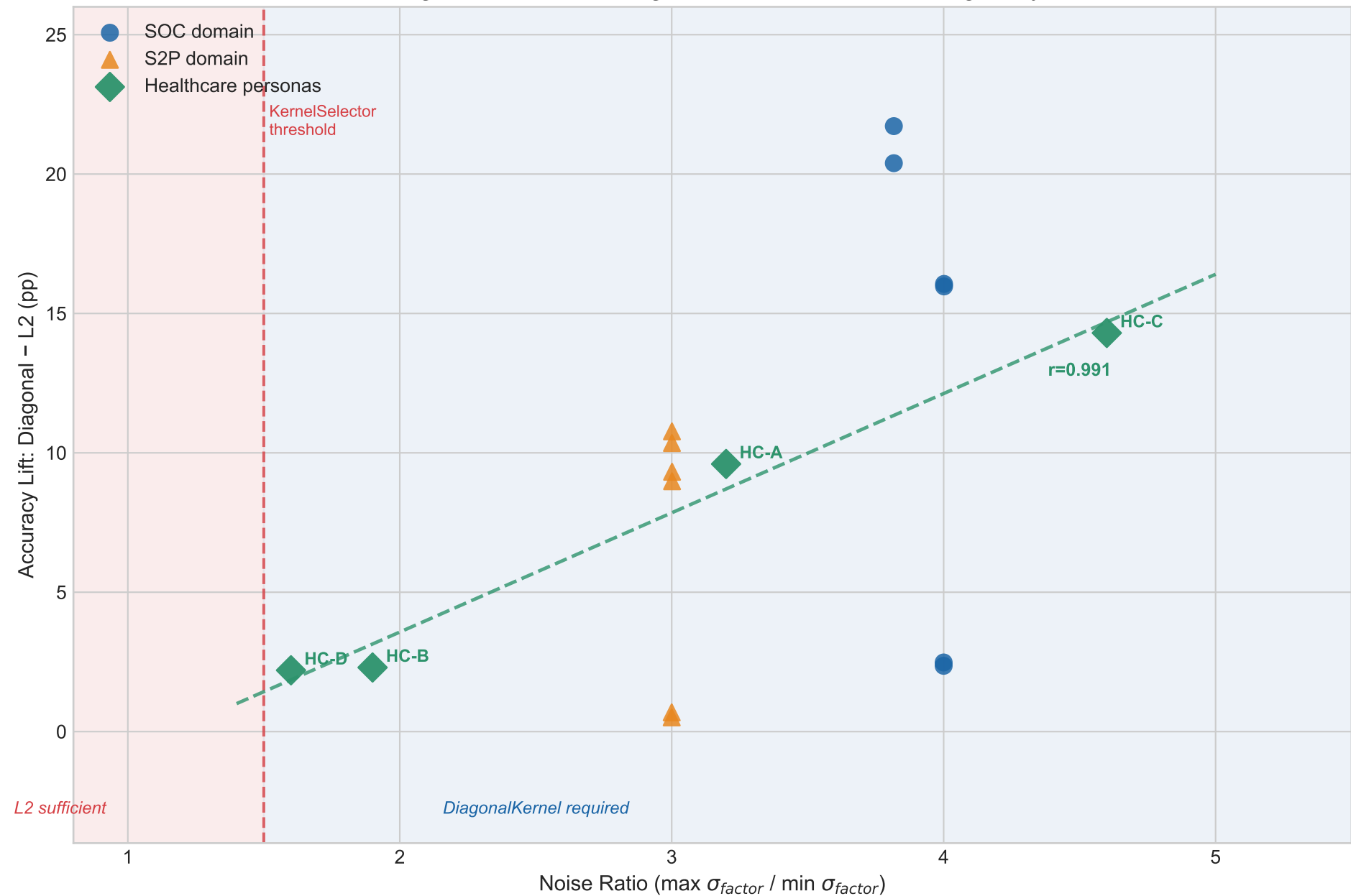
DiagonalKernel Advantage Scales with Noise Heterogeneity
