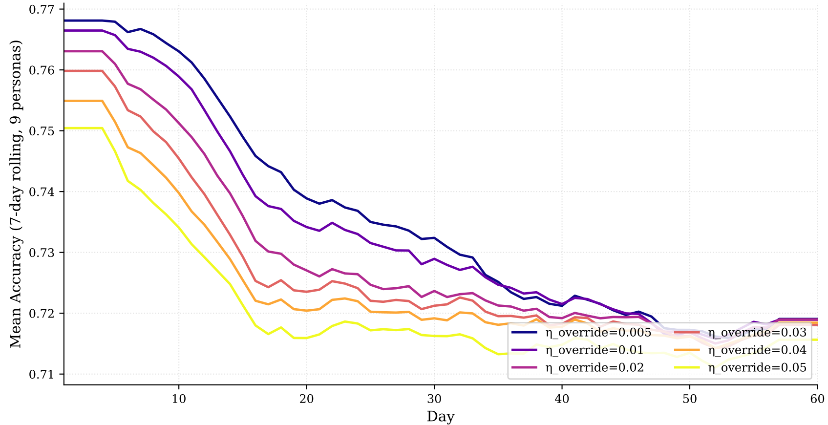
Accuracy Trajectories by Override Learning Rate
