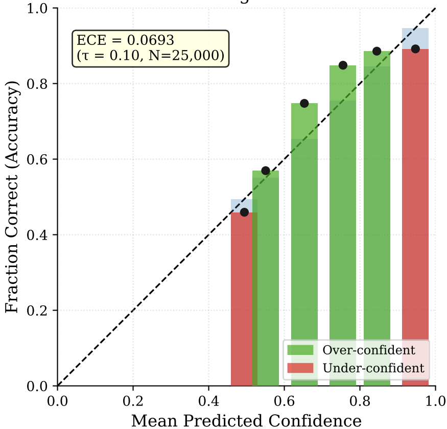
Calibration Diagram at \tau = 0.10
