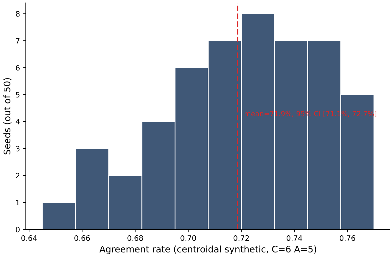
PROD-3: Shadow mode agreement rate distribution
