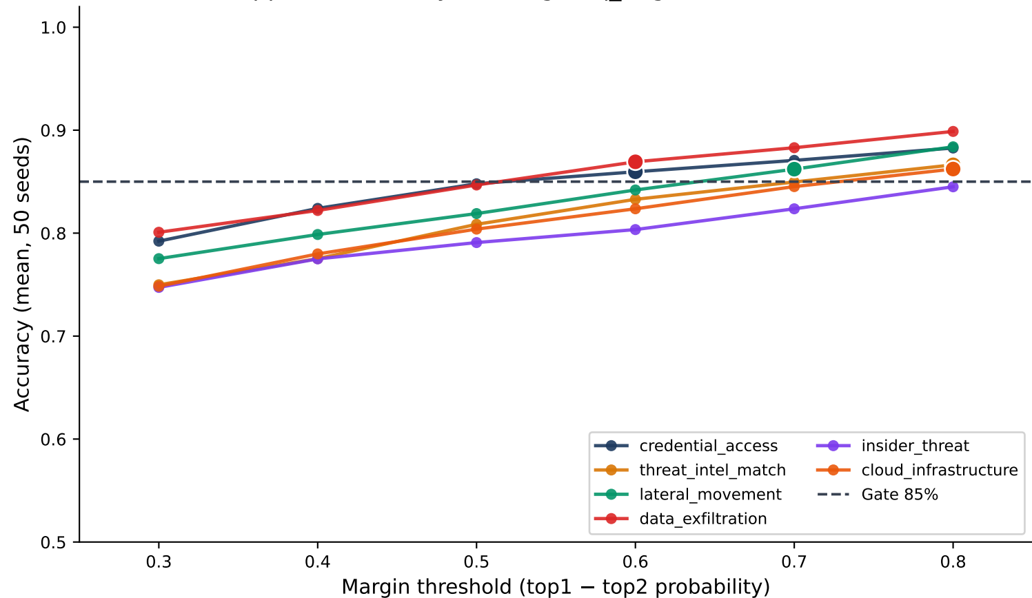
Auto-approve accuracy vs margin ( \eta_{\text{neg}}=0.05 , 50 seeds, A=5 )
