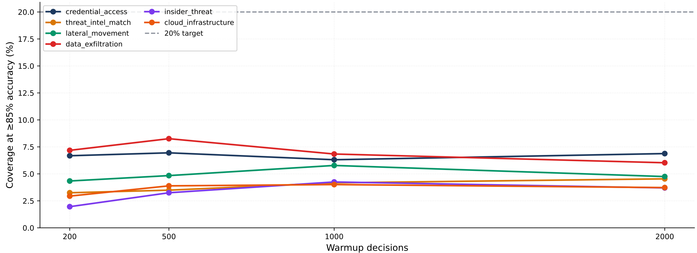
Auto-Approve Coverage Growth vs Warmup ( \eta_{\text{neg}}=0.05 , \tau=0.1 , 50 seeds, centroidal synthetic)
