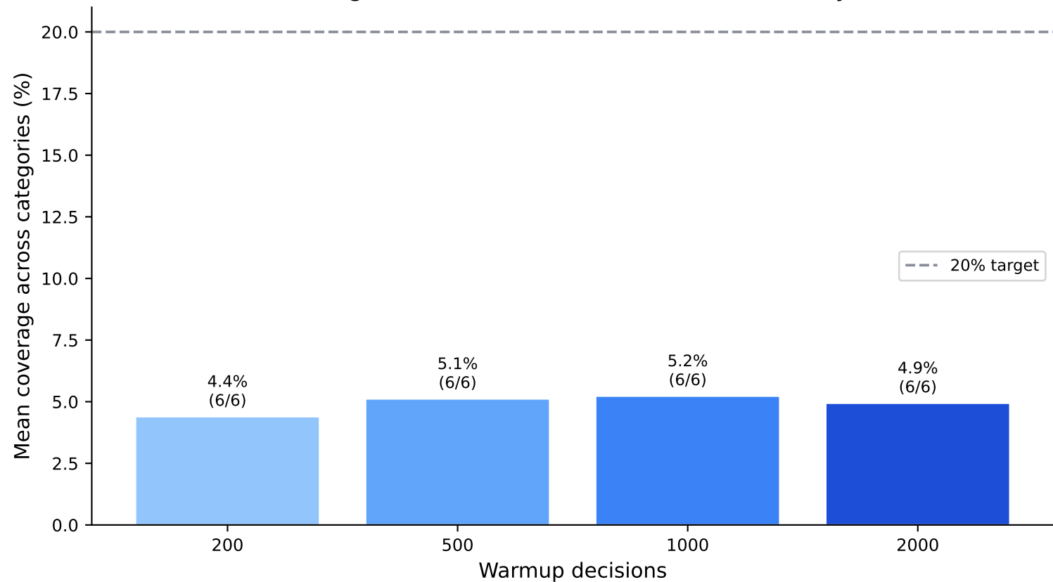
Mean Auto-Approve Coverage vs Warmup (categories with threshold* at \geq 85\% accuracy)
