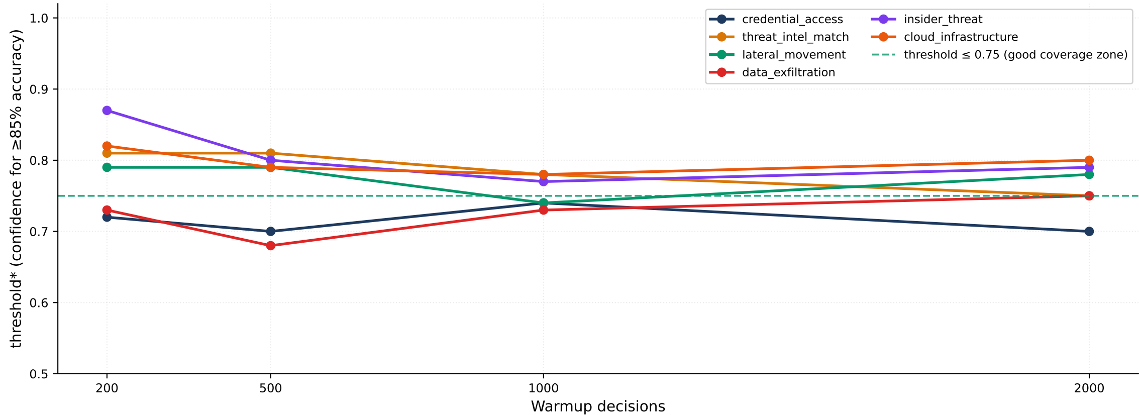
Threshold* Descent with Warmup (lower threshold* = more decisions auto-approved at same accuracy)
