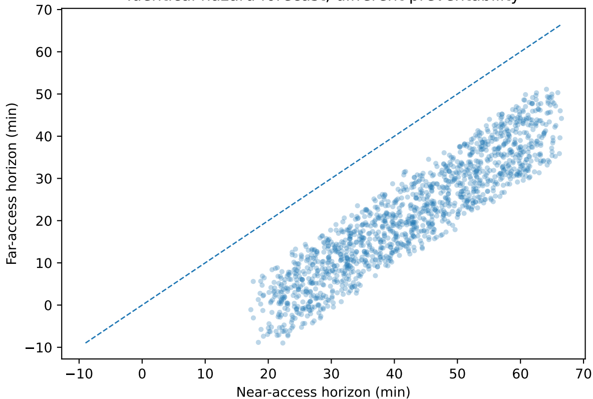
Identical hazard forecast, different preventability
