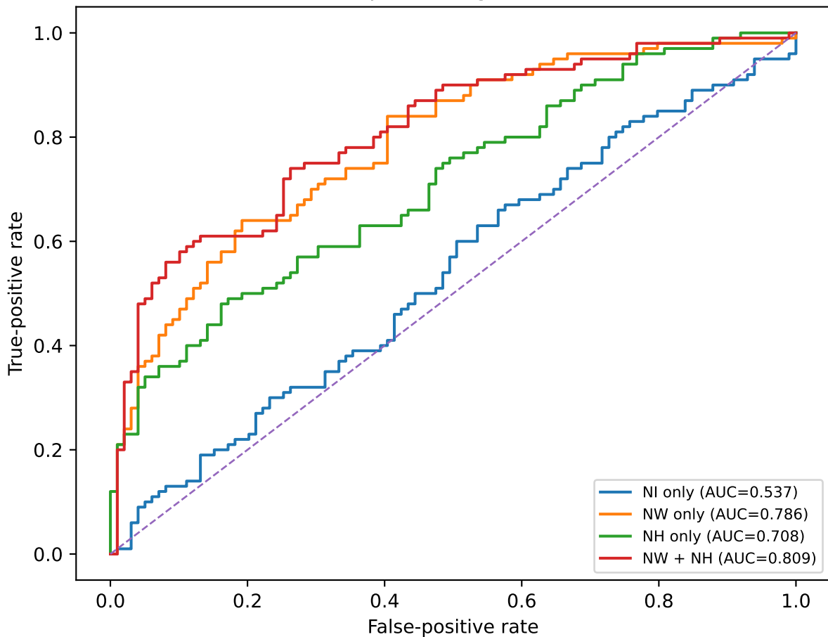
Information-preserving feature ablation
