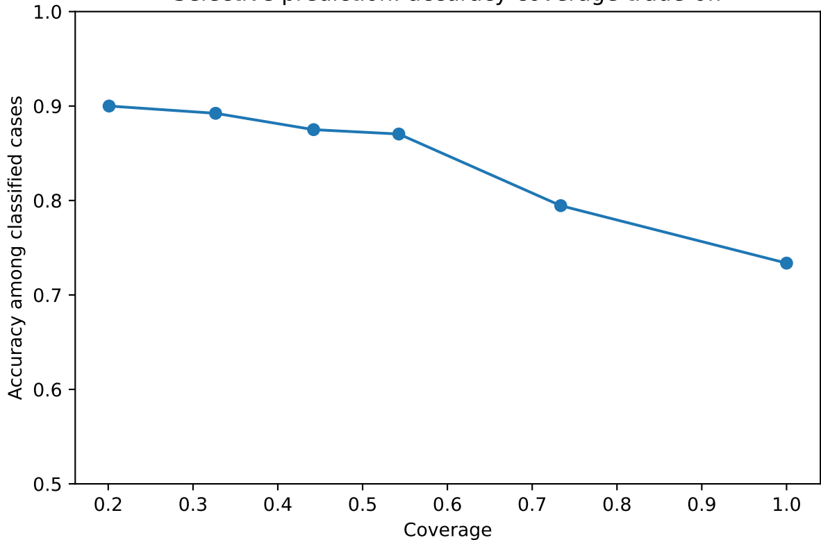
Selective prediction: accuracy-coverage trade-off
