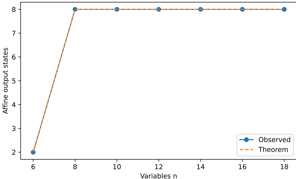
Proper-affine semantic image: exhaustive verification
