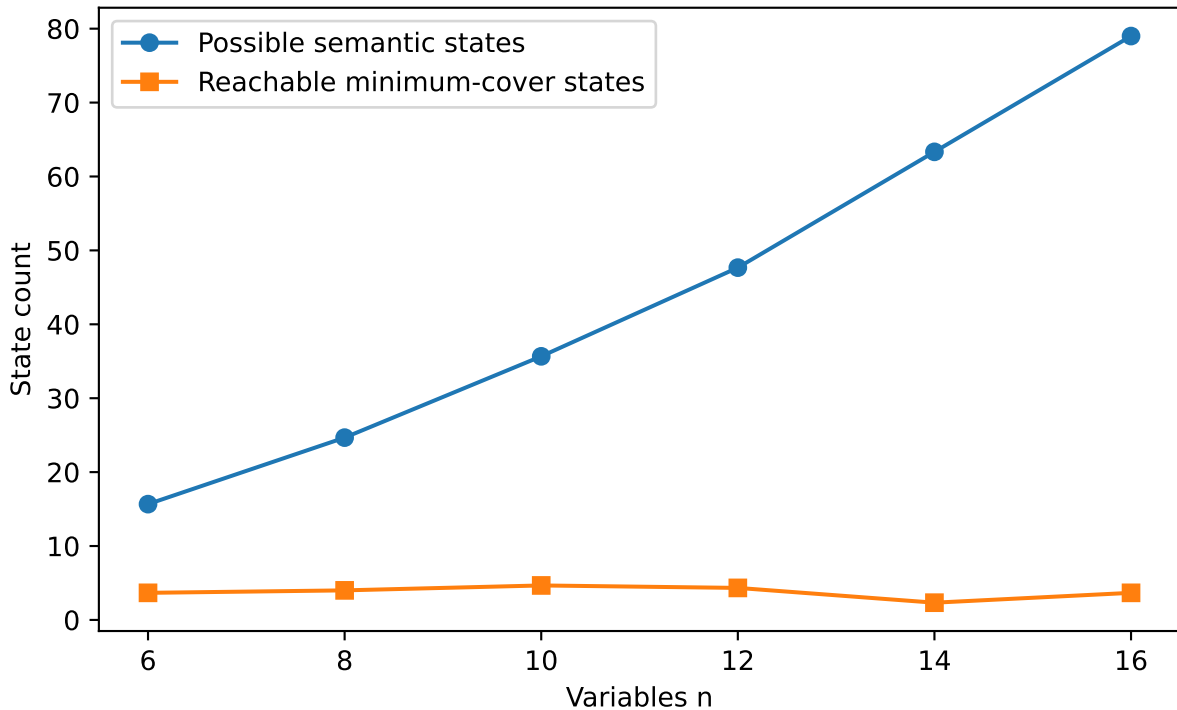
Finite semantic-resolution barrier diagnostic
