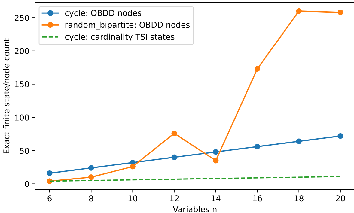
Finite OBDD diagnostic vs task-semantic states
