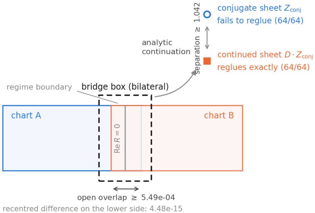
Figure 4: Continuation across a certified bridge: open overlap, regime boundary, and the conjugate sheet versus the continued sheet D \cdot Z_{\text{conj}} . ( schematic, annotated with certified margins )
