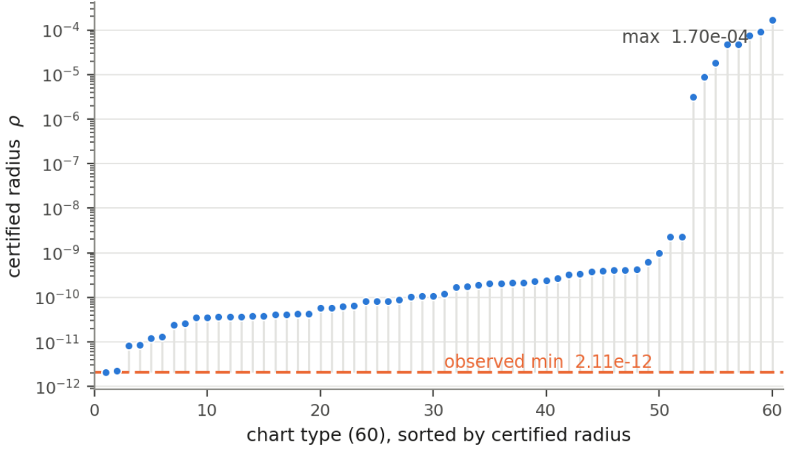
Figure 2: Certified radius across the 60 chart types on a log scale, spanning [2.11 \times 10^{-12}, 1.70 \times 10^{-4}] . The dashed line is the observed minimum over the types, 2.11 \times 10^{-12} ; the guaranteed floor quoted in the text, \rho_{\text{unif}} \geq 2.10 \times 10^{-12} , is that value rounded outward. Regenerated from the repaired chart certificate. (data)
