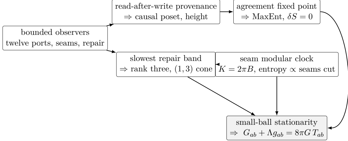
Figure 1: From bounded observers to the field equation. The left half is finite mathematics; the right half supplies the three inputs Jacobson’s derivation takes as given.
